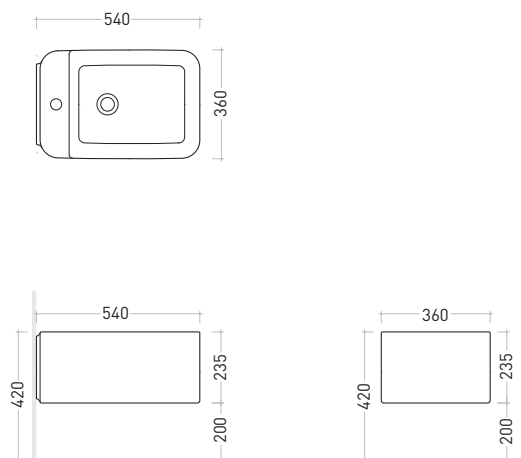
art. NL218 Bidet sospeso monoforo Wall hung single-hole bidet
