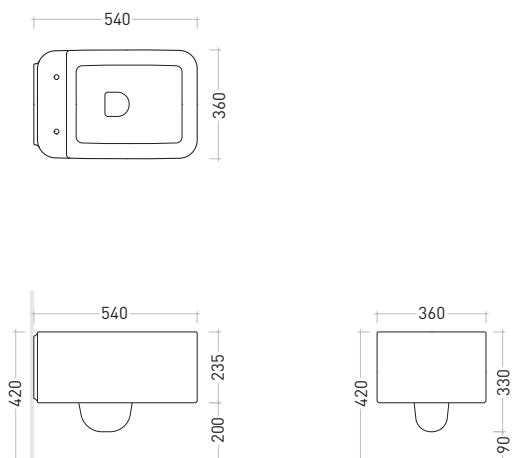
art. NL118 Vaso sospeso Wall hung wc
